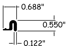
10 WEATHERSTRIP Q-LON
